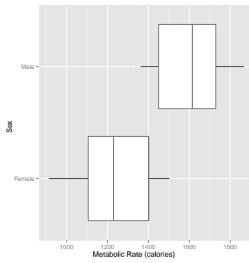
Figure 14: Boxplots of metabolic rate by sex for the data from BPS5 problem 4.9.
