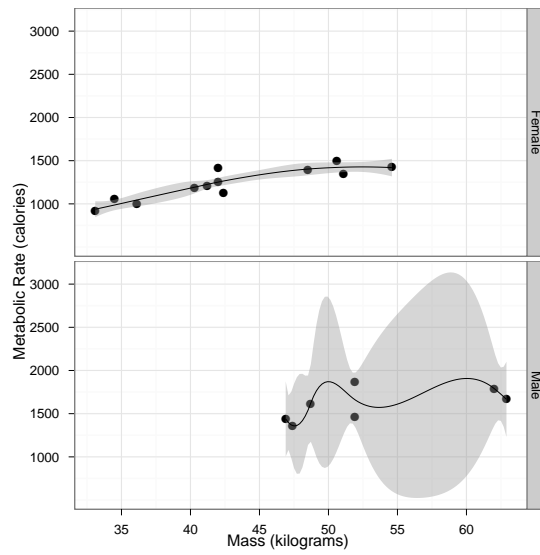
Figure 18: LOESS fits with approximate 95% confidence bounds for all data by sex.
