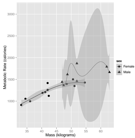
Figure 17: LOESS fits with approximate 95% confidence bounds for all data by sex.
