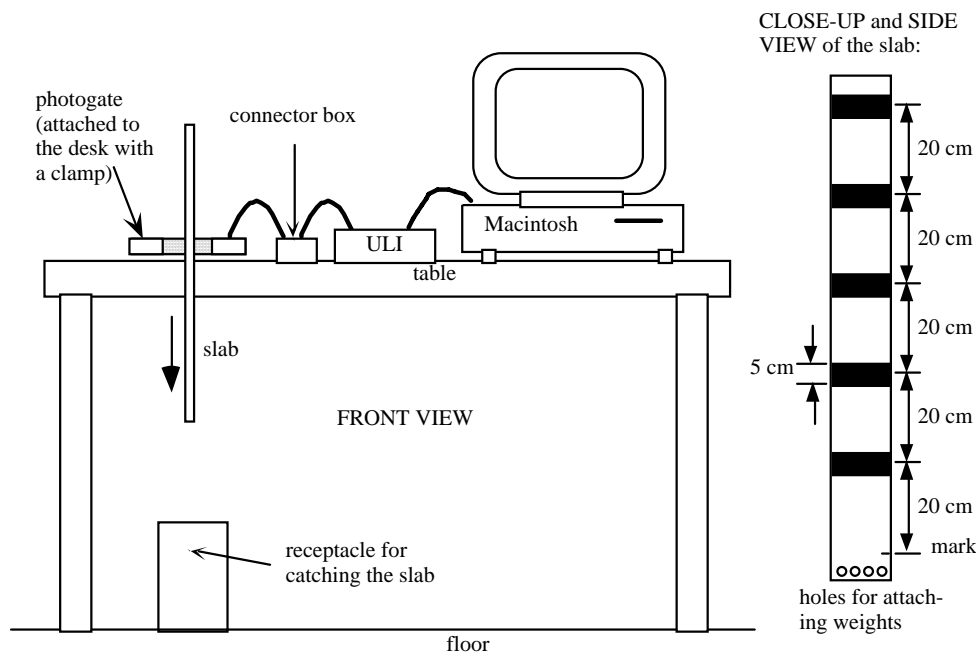
Figure 1: Sketch of the apparatus
